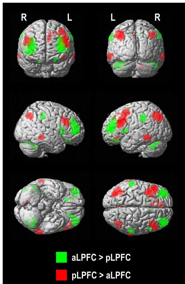
Fig. 3 Contrast between aLPFC and pLPFC RS-fMRI activation, showing regions where the effect of aLPFC was greater than pLPFC (green), and vice versa (red). Analysis was performed in MNI space
