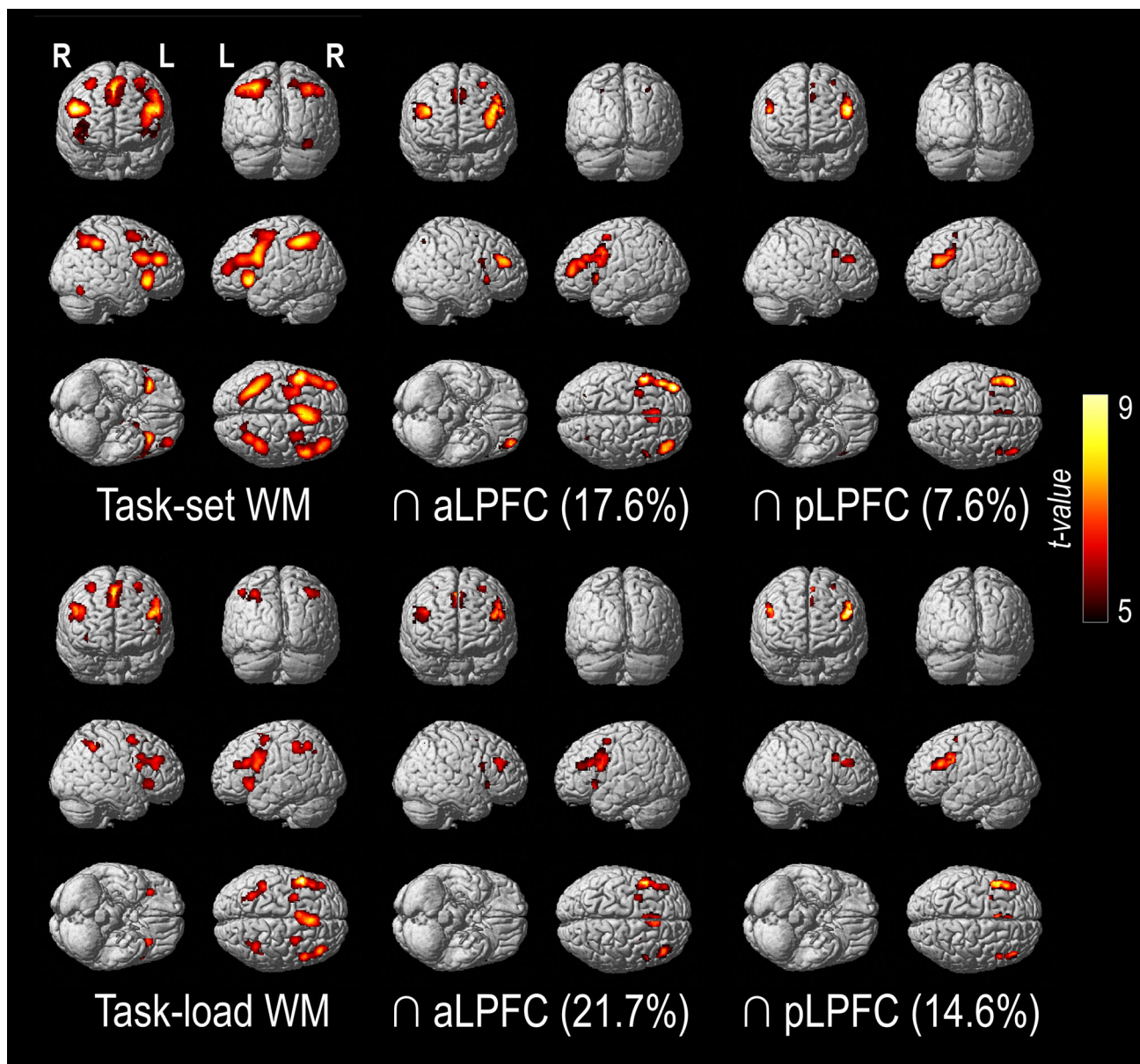
Fig. 4 Comparison of aLPFC and pLPFC connectivity to the working memory (WM) networks reported in Rottschy et al. (2012). Top the task-set network is an ALE distribution of studies contrasting WM task with a baseline or other control condition. At right, a conjunction of the task-set network with the cross-modal conjunctions shown in Fig. 2. Bottom a conjunction of the task-set network and a second ALE analysis contrasting high- and low-load
